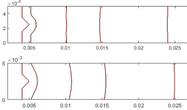
FIG. 2.2. Example 1: Time evolution of the fraction of unburnt gas z computed by the ADP (top row) and SDP (bottom row) methods. In both figures, the detonation wave propagates from left to right and the interface between the burnt and unburnt fractions of the gas is shown at times t=0, 10^{-8}, 5 \cdot 10^{-8}, 9 \cdot 10^{-8} and 1.7 \cdot 10^{-7} .
