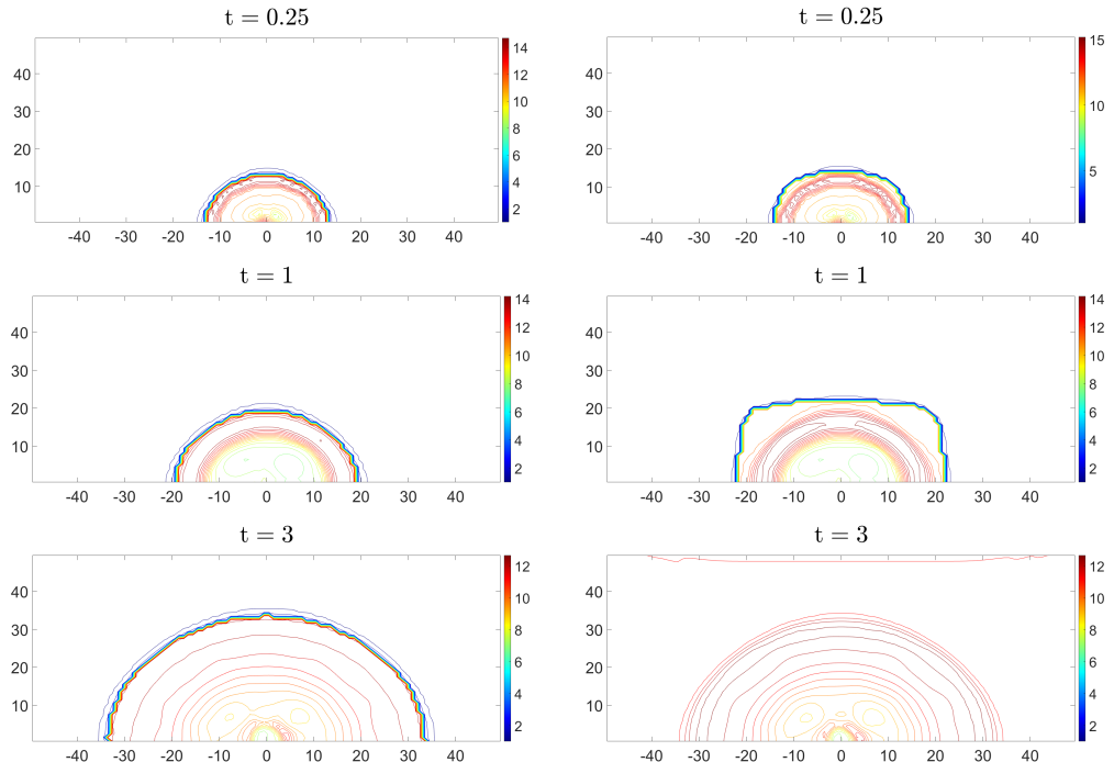
FIG. 2.3. Example 2: Temperature \tau computed by the ADP (left column) and SDP (right column) methods.
