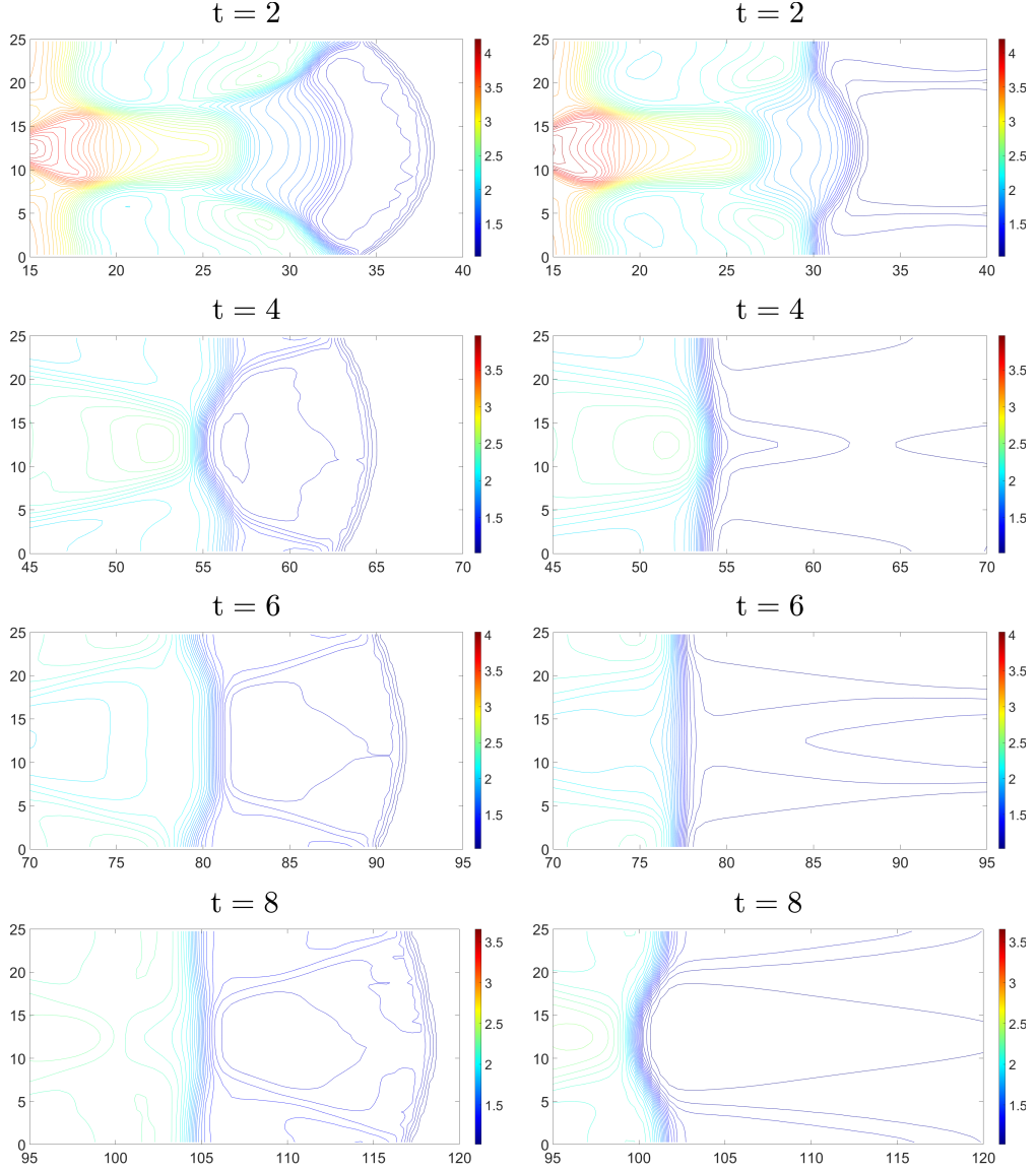
FIG. 4.13. Example 9c: Contour plots of density ( \rho ) computed by the ADP (left column) and SDP (right column) methods at different times.
