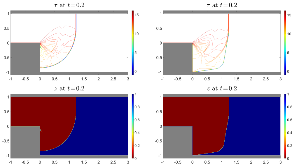
FIG. 2.8. Example 4: Temperature \tau (top row) and fraction of unburnt gas z (bottom row) at time t=0.2 computed by the ADP (left column) and SDP (right column) methods.
