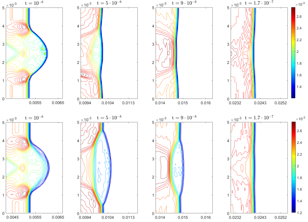
FIG. 2.1. Example 1: Density \rho computed by the ADP (top row) and SDP (bottom row) methods.
