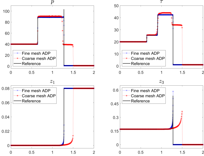
FIG. 4.8. Example 9b: Pressure ( p ), temperature ( \tau ), mass fraction of H_2 ( z_1 ) and mass fraction of OH ( z_3 ) computed by the ADP method with \Delta x = 1/150 and 1/600 for 1/\varepsilon_1 = 1/\varepsilon_2 = 10^6 .
