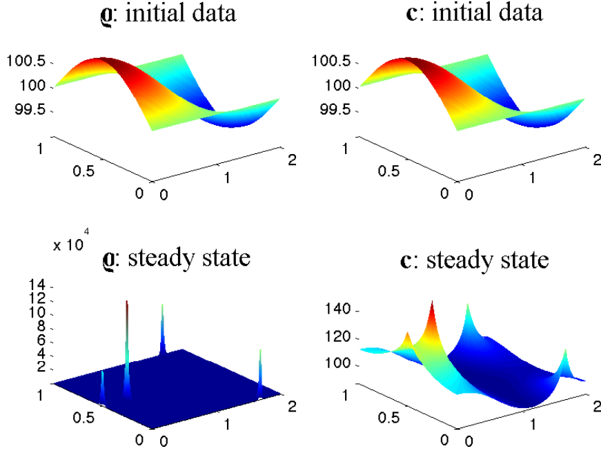
FIGURE 14. Four-spike structure emerging out of the initial data (104) using \Delta x = \Delta y = 1/100 .
