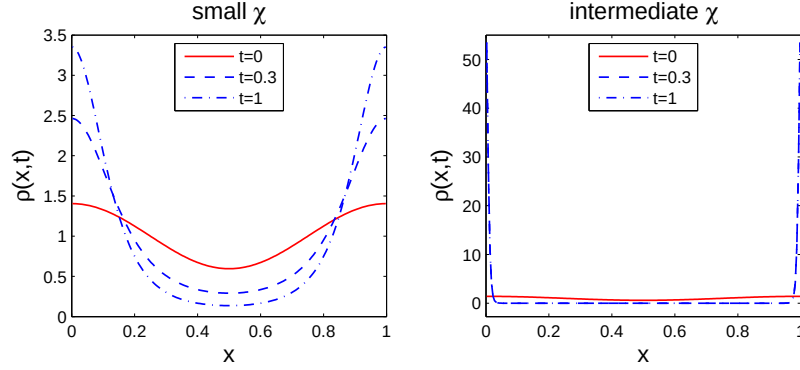
FIGURE 8. Double boundary spike steady states.
