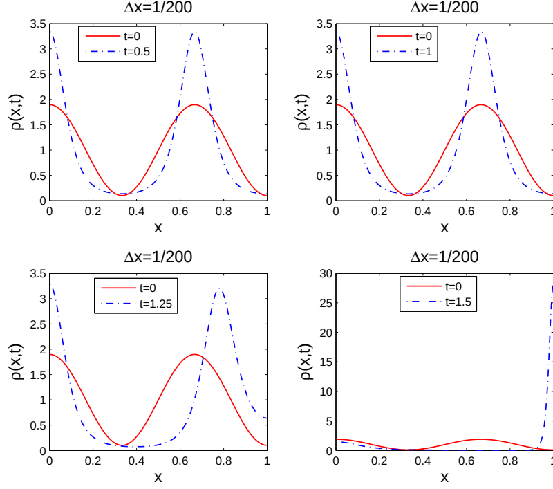
FIGURE 11. Numerical solution of the IVP (77), (55), (100). Solution symmetry is destroyed on a grid with \Delta x = 1/200 .
