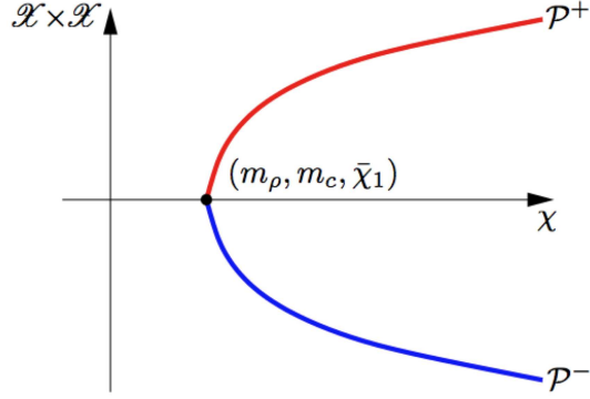
FIGURE 5. A bifurcation curve illustrating Theorem 5.3.
