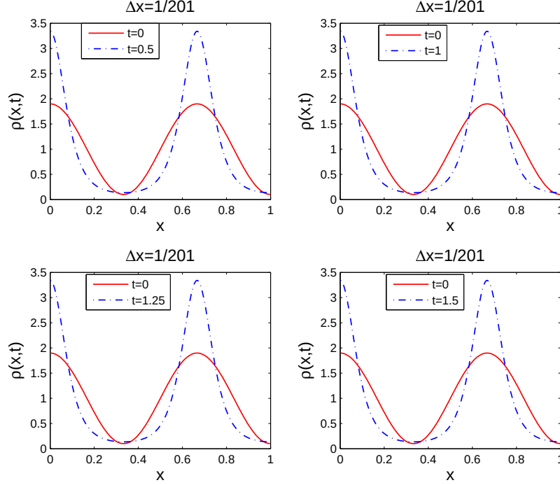
FIGURE 10. Numerical solution of the IVP (77), (55), (100). Solution symmetry is preserved on a grid with \Delta x = 1/201 .
