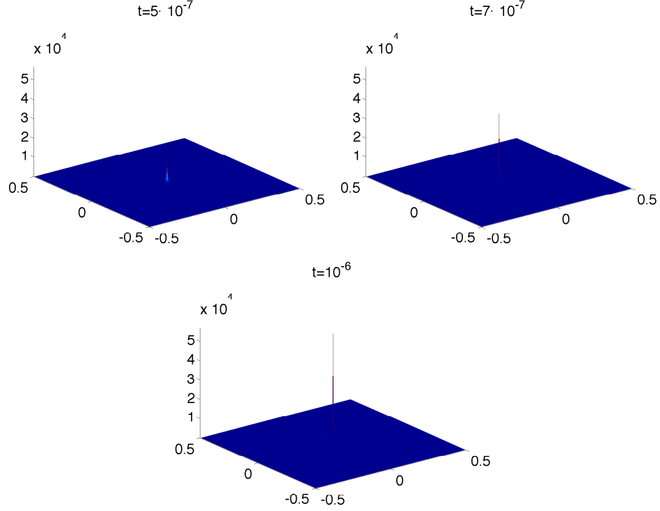
FIGURE 4. Numerical solution (\rho) of (1), (52).
