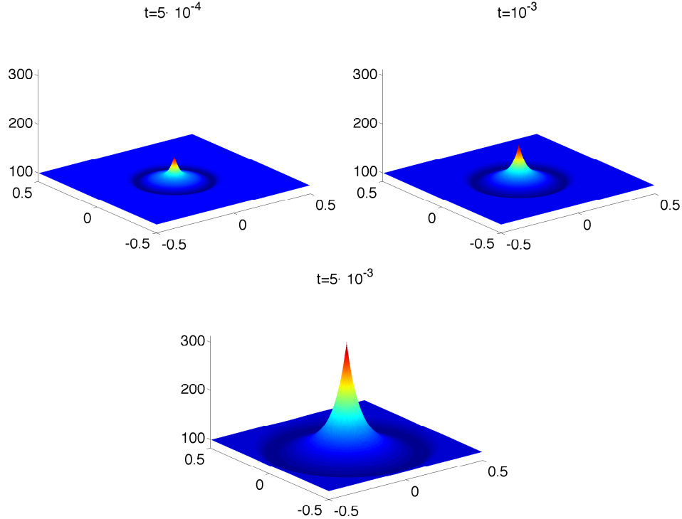
FIGURE 1. Numerical solution ( \rho ) of (2), (4), (52) with s^* = 0 .
