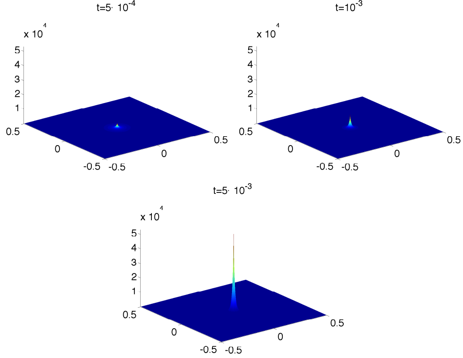
FIGURE 3. Numerical solution (\rho) of (2), (4), (52) with s^* = 10 .
