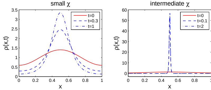
FIGURE 9. Single interior spike steady states.
