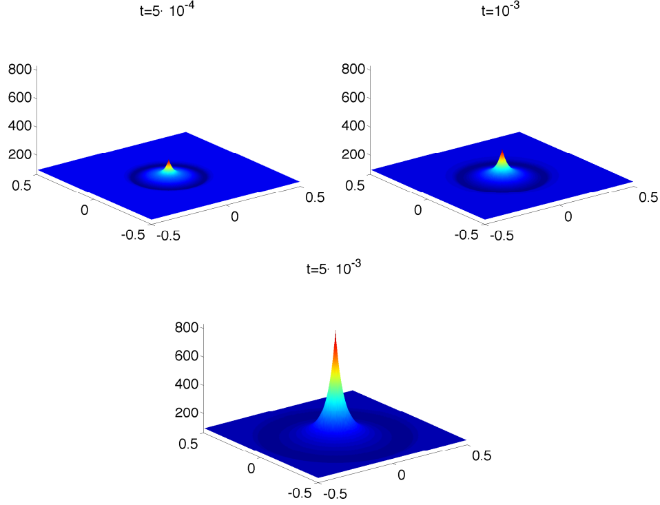
FIGURE 2. Numerical solution (\rho) of (2), (4), (52) with s^* = 1 .
