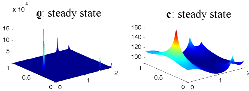
FIGURE 15. Five-spike structure emerging out of the initial data (104) using \Delta x = 2/201, \Delta y = 1/101 .
