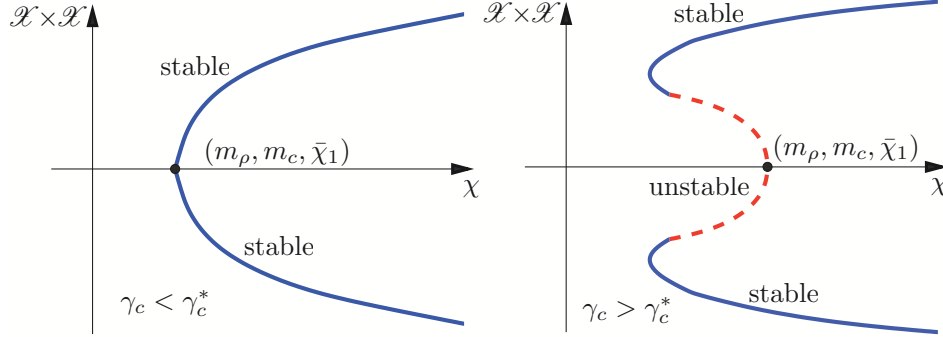
FIGURE 7. Stable (solid line) and unstable (dashed line) parts of typical bifurcation curves.
