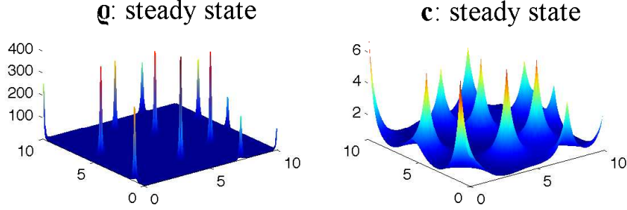
FIGURE 16. Multi-spike structure emerging out of the random initial data (105).
