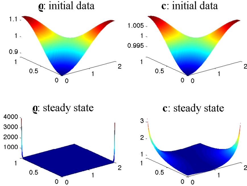
FIGURE 12. Double corner spike emerging out of the symmetric initial data (102).
